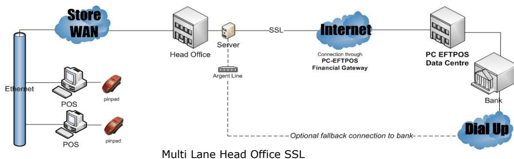
The above diagrams show examples of small and large scale businesses, connecting through the PC-EFTPOS IP Communications Gateway. These solutions offer the flexibility of using a fallback option when the internet connection is down.
